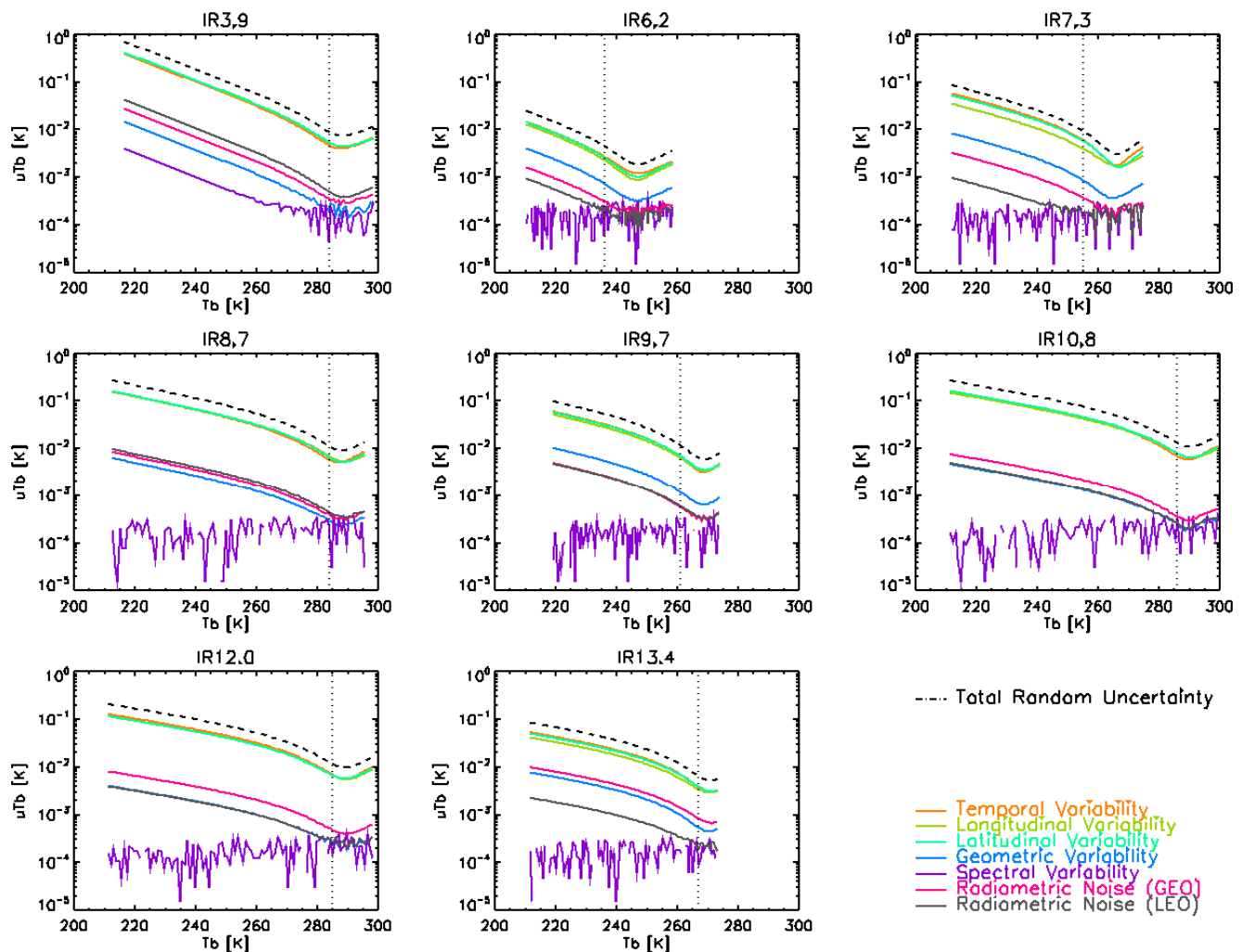
Fig. 2. Contribution of each source of random error, u_j^r(\hat{L}) , to the standard uncertainty of the brightness temperatures ( T_b ) produced by the GSICS Correction for a range of scene radiances for each infrared channel of Meteosat9/SEVIRI using Metop/IASI reference. Dotted vertical line shows standard radiance for each channel, corresponding to nadir views of a calm ocean in clear standard atmosphere conditions.
