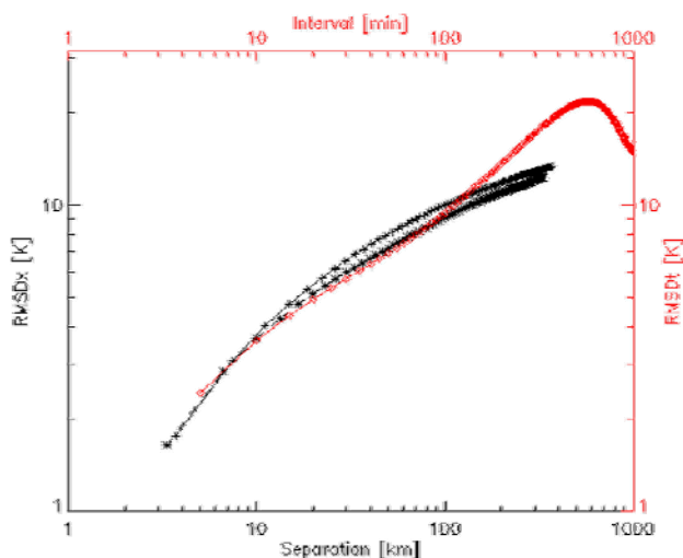
Fig. A-1. Variograms calculated as RMS differences in Meteosat-8/SEVIRI 10.8 \mu\text{m} brightness temperatures with time intervals from Rapid Scanning data (red diamonds, upper x-axis) and with spatial separation in North-South direction (black pluses, lower x-axis) and West-East direction (black
