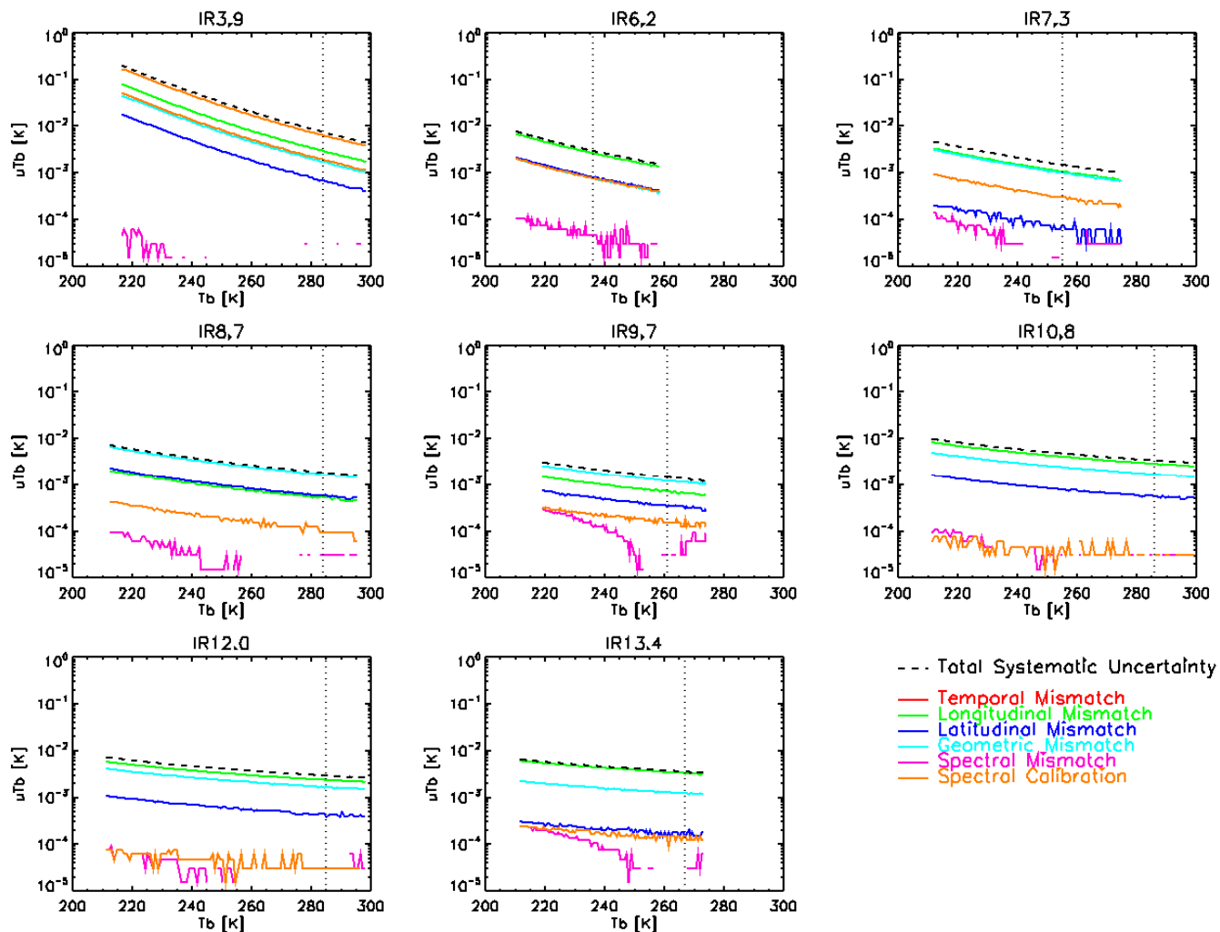
Fig. 1. Contribution of each source of systematic error, u_j^s(\hat{L}) , to the standard uncertainty of the brightness temperatures ( T_b ) produced by the GSICS Correction for a range of scene radiances for each infrared channel of Meteosat9/SEVIRI using Metop/IASI reference. Dotted vertical line shows standard radiance for each channel, corresponding to nadir views of a calm ocean in clear standard atmosphere conditions.
