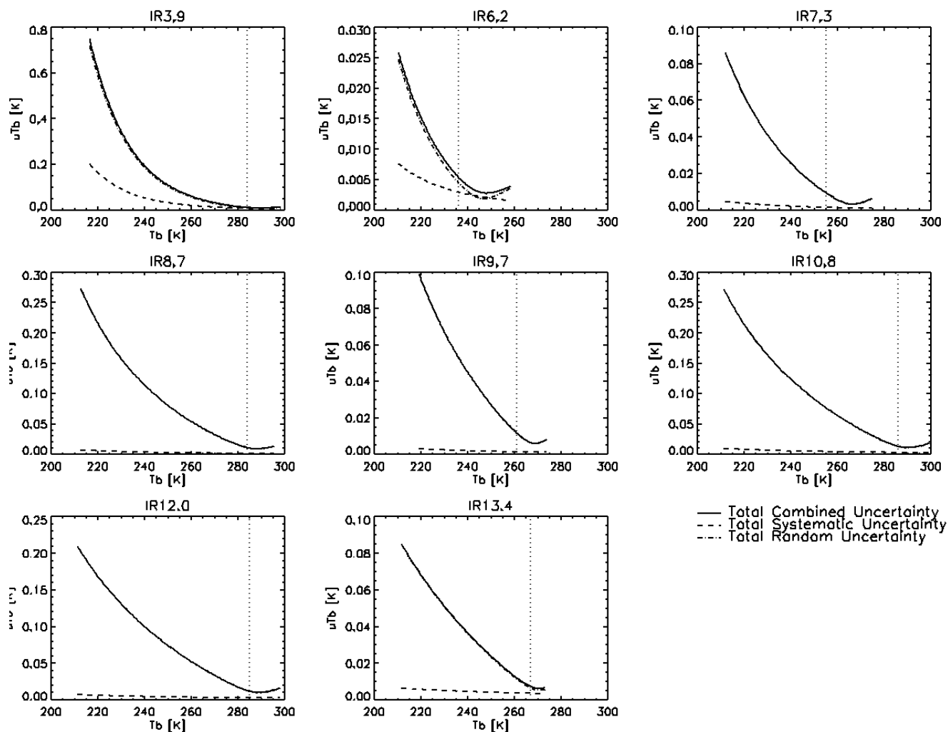
Fig. 3. Impact of total systematic, u^s(\hat{L}) , random, u^r(\hat{L}) , and combined, u^c(\hat{L}) , errors on ( k=1 ) uncertainty of the brightness temperatures ( T_b ) produced by the GSICS Correction for a range of scene radiances for each infrared channel of Meteosat9/SEVIRI using IASI reference. Dotted vertical line shows standard radiance for each channel.
